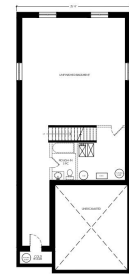
BASEMENT PLAN
