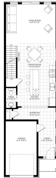
MAIN FLOOR
