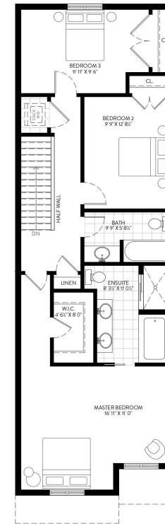
SECOND FLOOR
